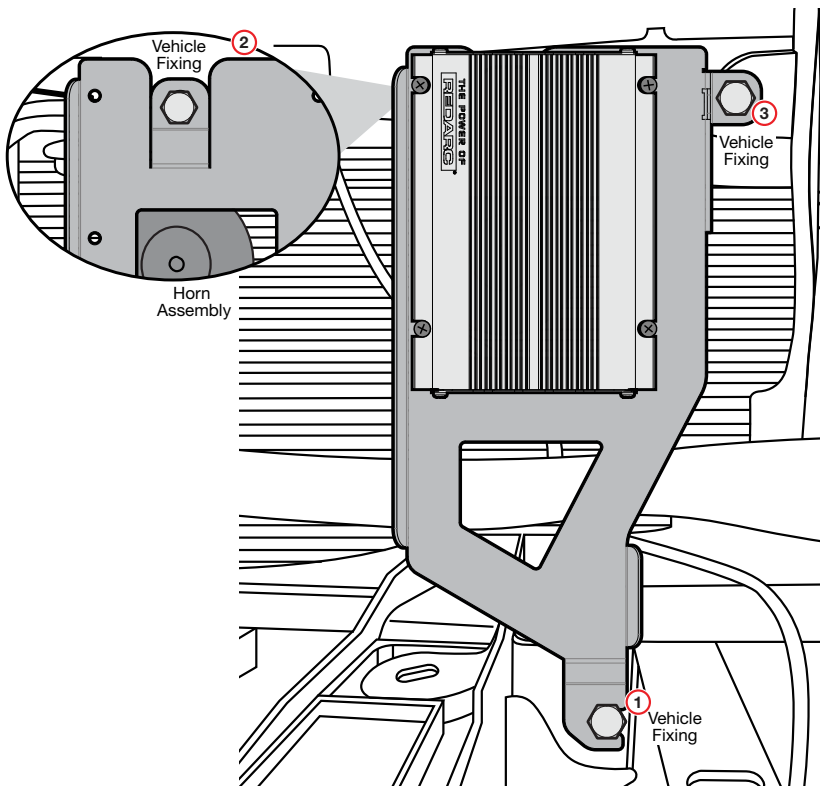
Figure 5: Securing Mounting Bracket to Vehicle
