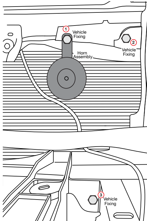
Figure 4: Removing Vehicle Fixings
